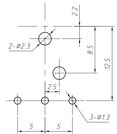
Mounting Hole
