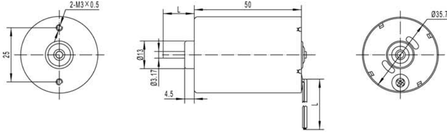
Motor Dimensions (mm)
