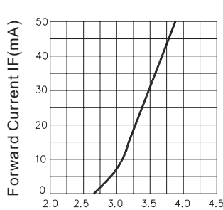
Forward Voltage VF(V) Fig.2 Forward Current vs. Forward Voltage
