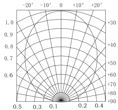
Emitted Angle 100°
