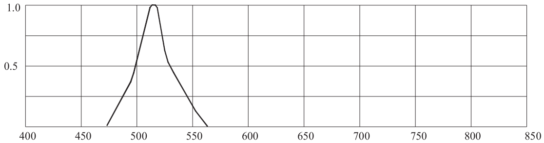
Wavelength \lambda (nm) Fig. 1 Relative Intensity vs . Wavelength
